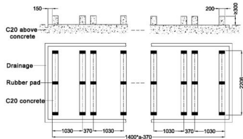
b. Concrete foundation diagram
