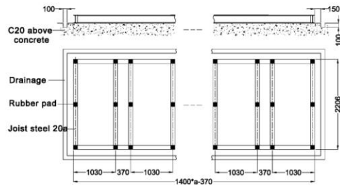
a. Joist steel foundation diagram
