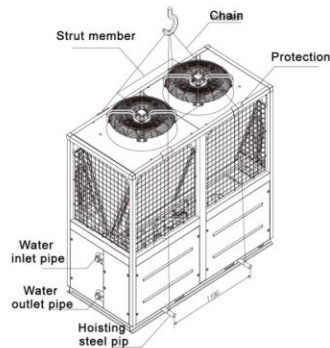
Example lifting schematic for TCA201
