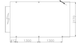
Base vibration absorption installation diagram 6-φ14 vibration absorption installation hole
