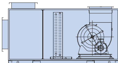
Mixing box (include nylon filter) + coil + fan
