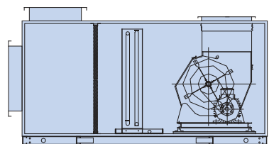
Mixing box (include panel filter) + coil + fan
