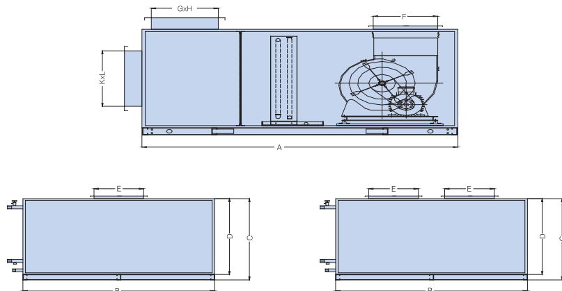
Standard unit one, two (with pre-filter)
