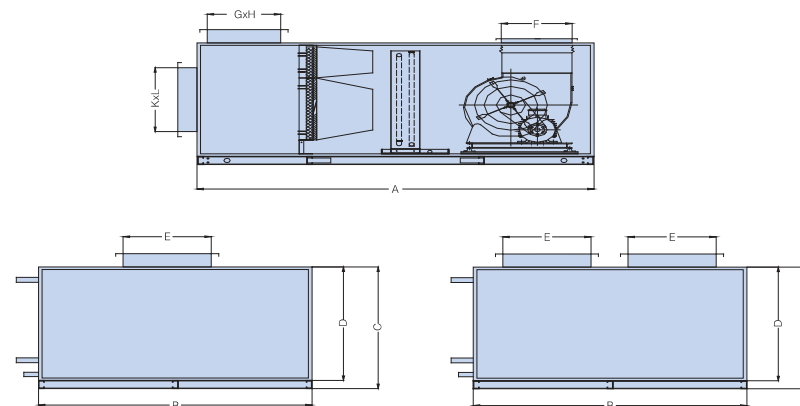
Standard unit three (with pre-filter & medium filter)
